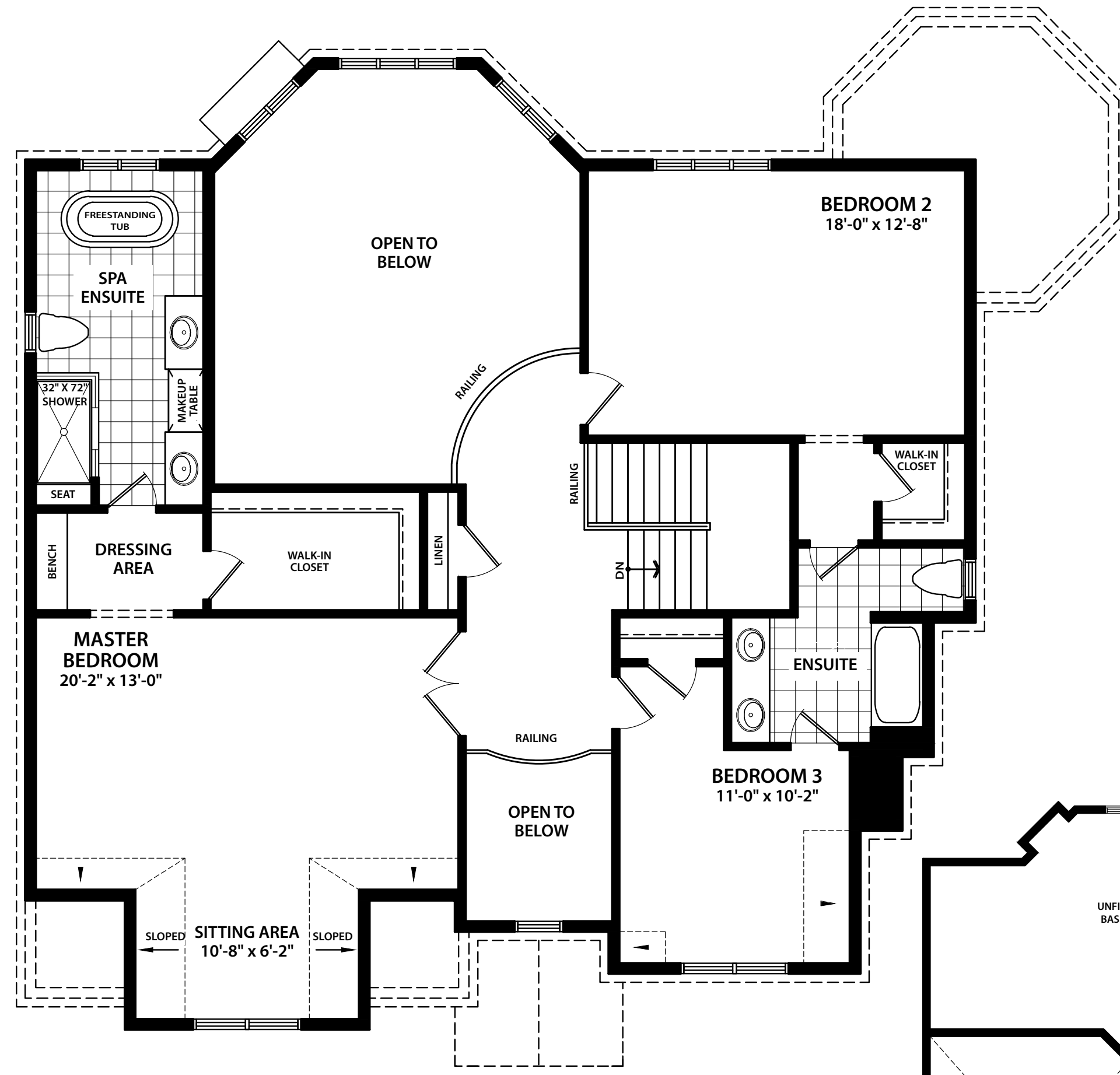
SECOND FLOOR
