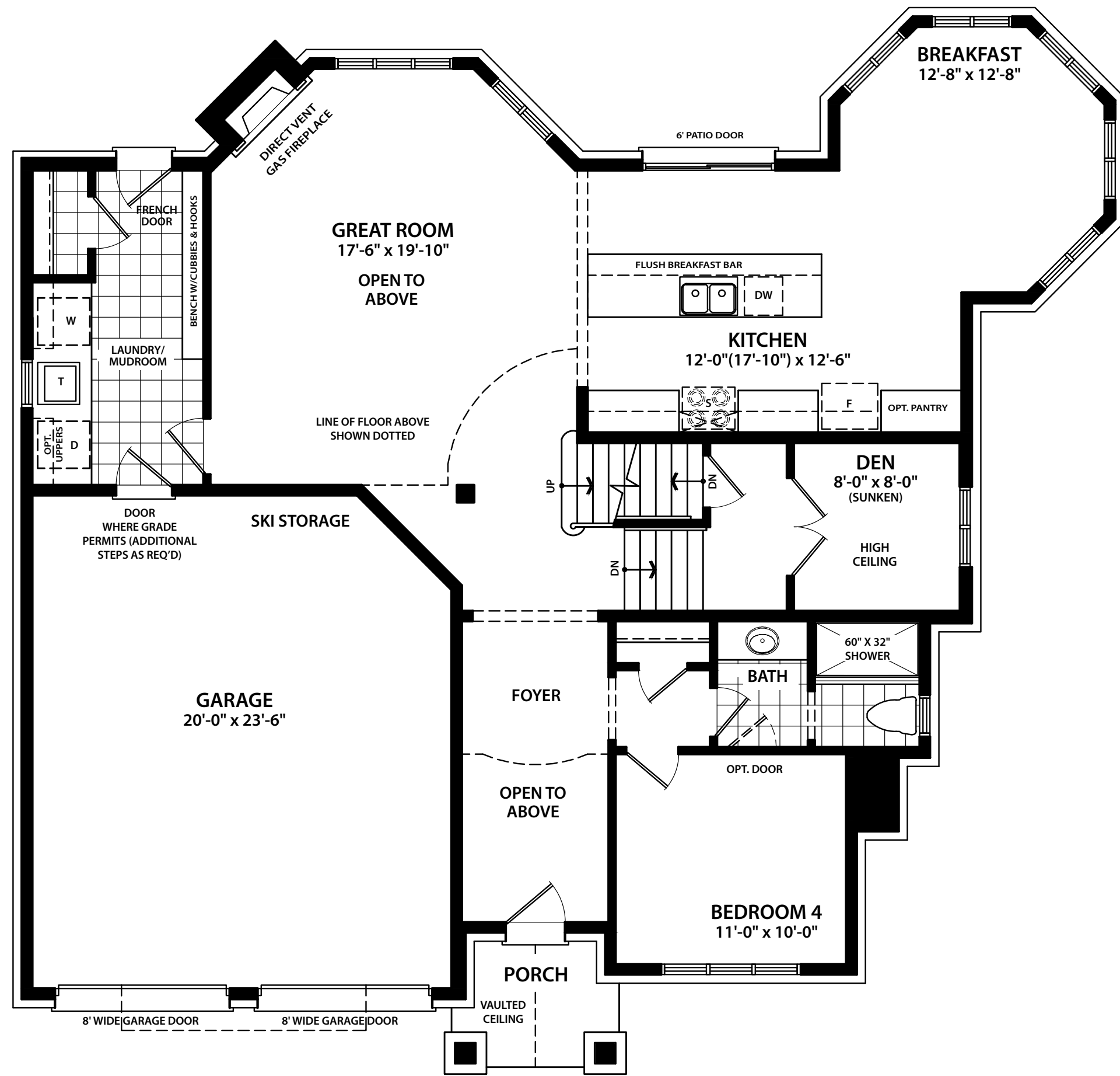
GROUND FLOOR
